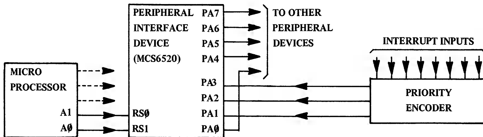
Priority Encoder to Peripheral Interface Scheme
